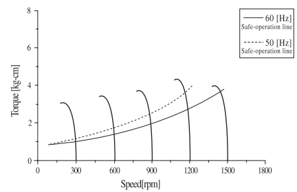
Single phase L9R40□□LT
